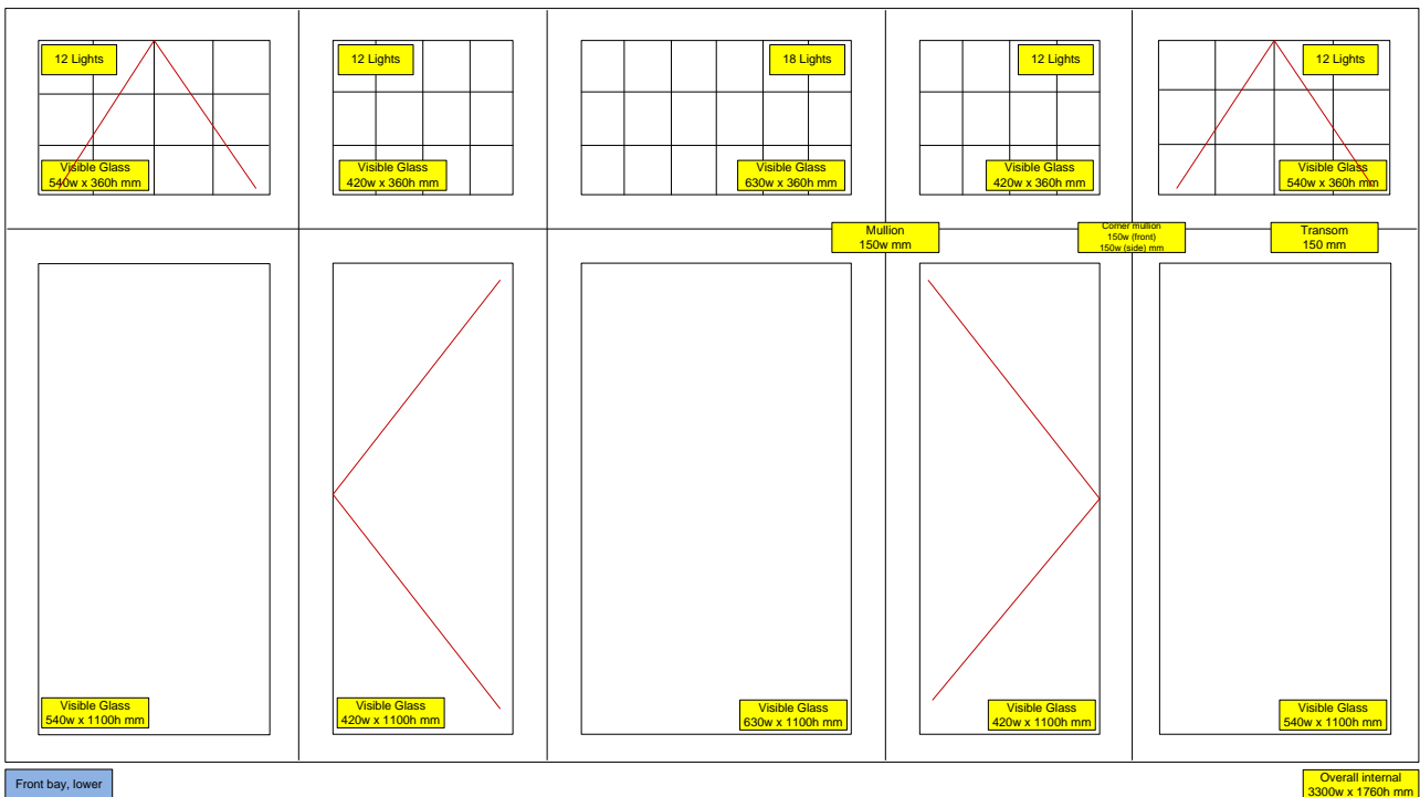
Front Elevation Ground Floor Bay – Lounge
