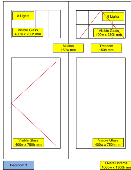
Front Elevation First Floor – Bedroom 3
