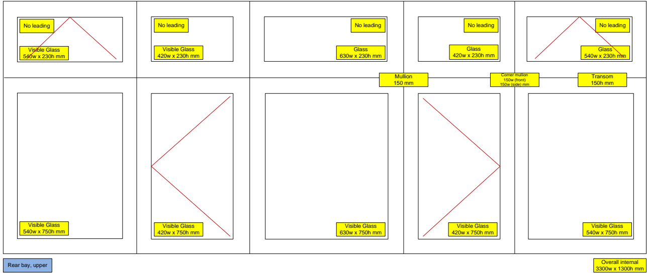
Rear Elevation First Floor Bay – Bedroom 2
