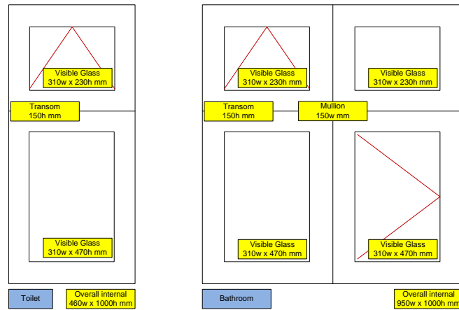
Side Elevation First Floor – Bathroom and Toilet
