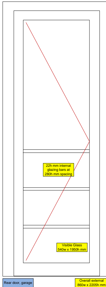
Rear Elevation Ground Floor – Garage Door
