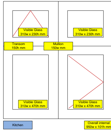
Side Elevation Ground Floor – Kitchen
