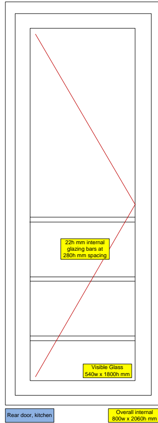
Rear Elevation Ground Floor – Kitchen Door
