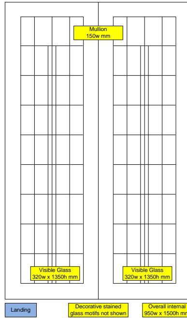
Side Elevation First Floor – Landing
