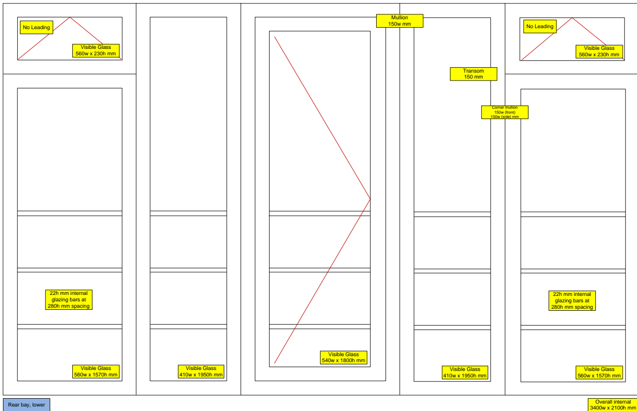
Rear Elevation Ground Floor Bay – Lounge
